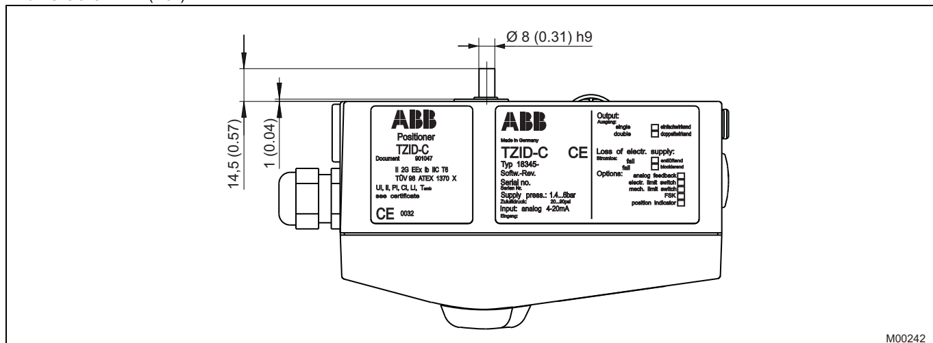
Fig. 9: Top view
