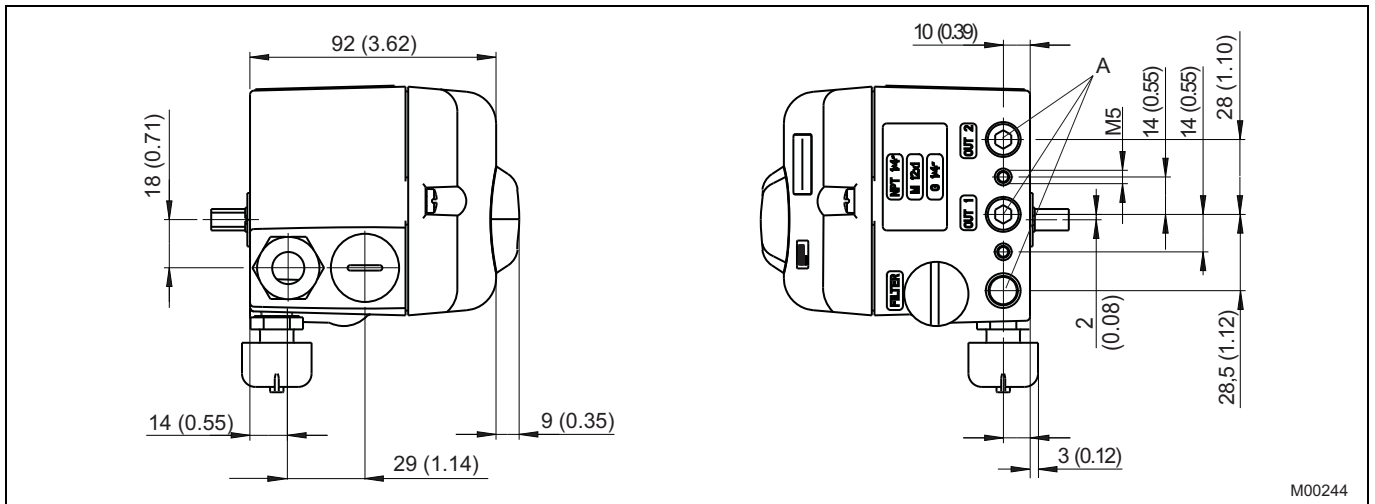
Fig. 11: side view (from left to right) A Pneumatic connections, NPT 1/4"-18 or G1/4"
