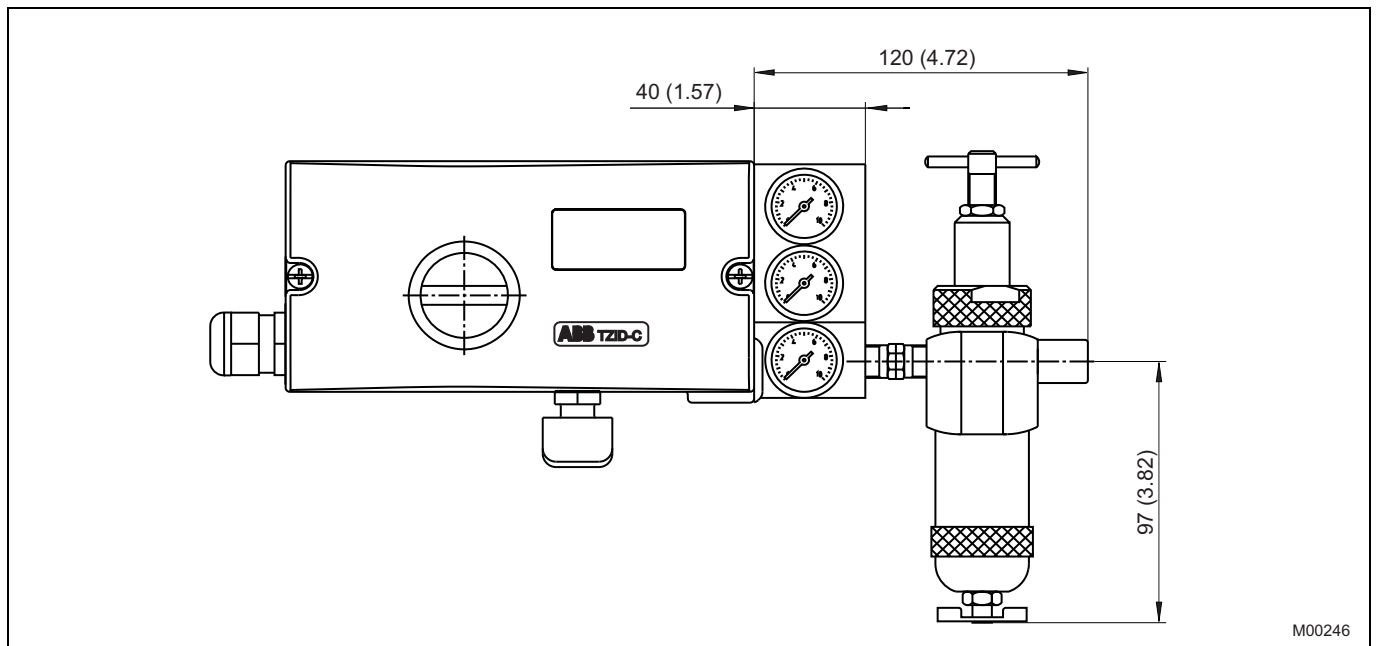
Fig. 13: Positioner with pressure gauge block and filter regulator
